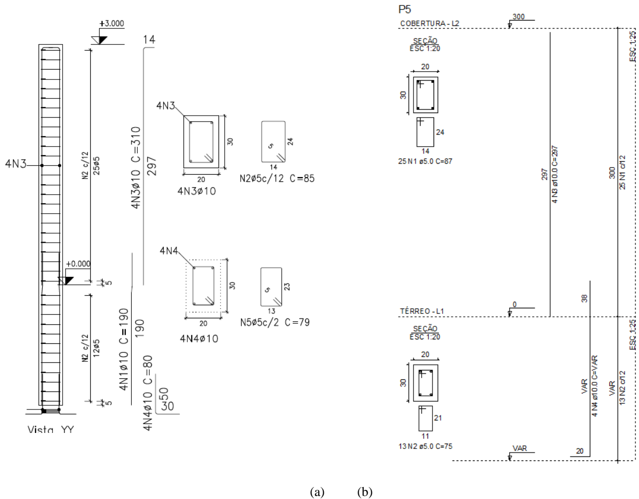
Figura 12 – Detalhes do pilar P5 – (a) Cypecad (b) Eberick.
