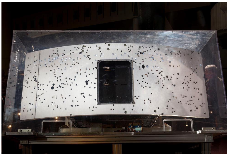
FIGURE 1: Rear-end extremity of the radiator onboard Wide Field Planetary Camera II (WFPC2), installed on the Hubble Telescope, by Eric Long, National Air and Space Museum.
