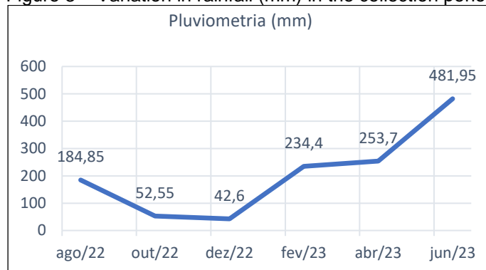
Figure 3 – Variation in rainfall (mm) in the collection period
