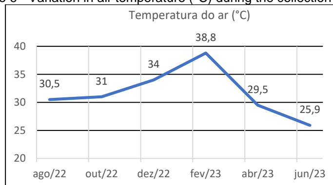
Figure 6 - Variation in air temperature (°C) during the collection period.
