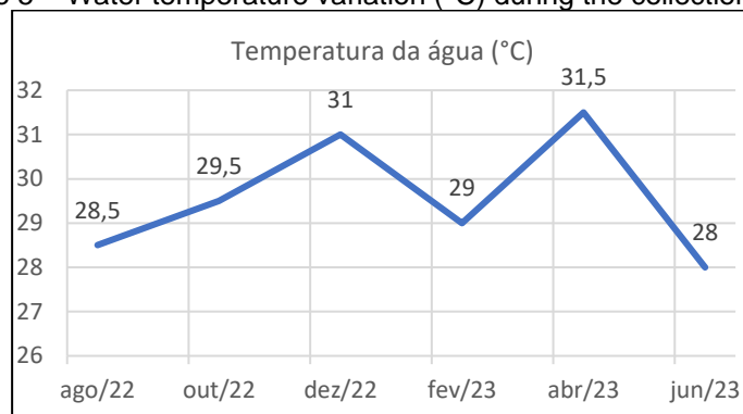
Figure 5 – Water temperature variation (°C) during the collection period
