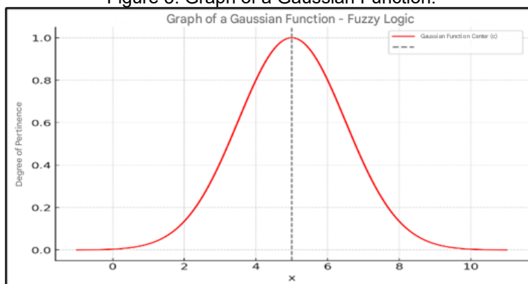
Figure 3: Graph of a Gaussian Function.
