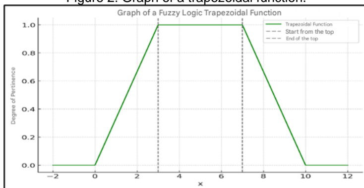
Figure 2: Graph of a trapezoidal function.
