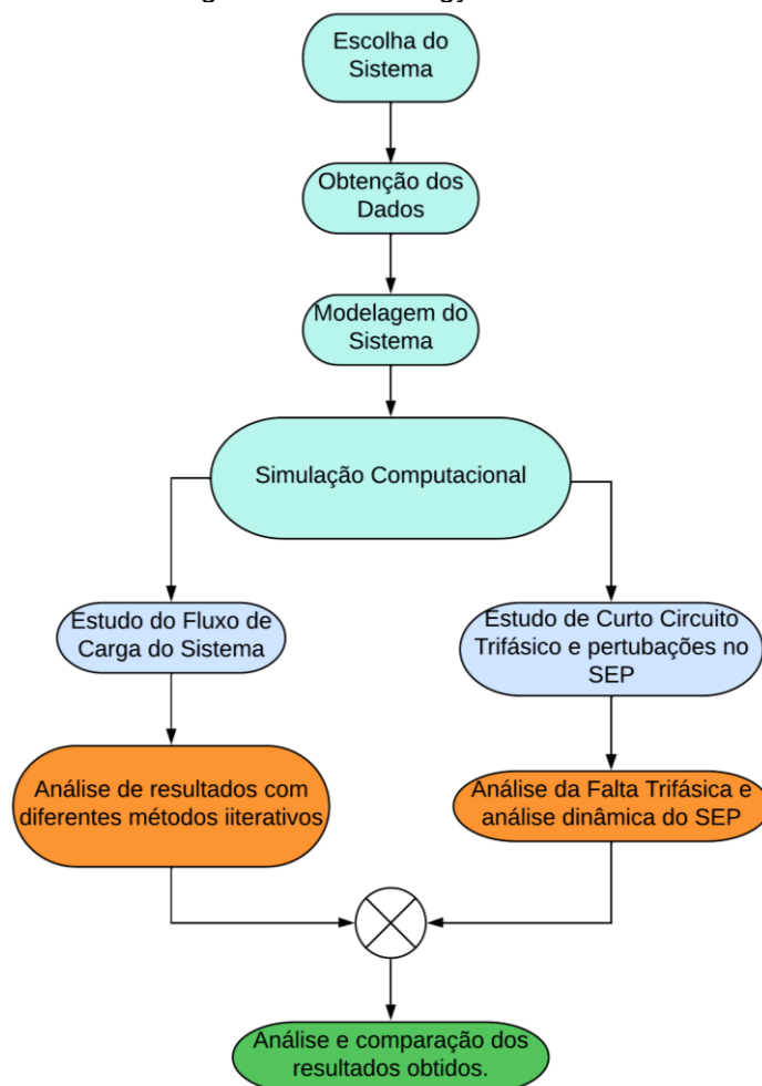
Figure 1: Methodology flowchart.
