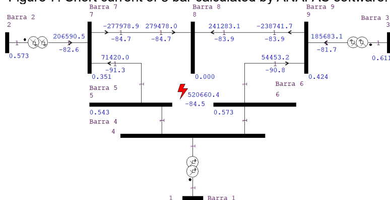
Figure 7: Short current of 8 bar calculated by ANAFAS software.
