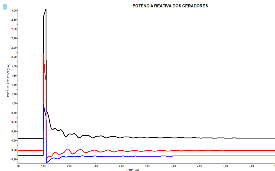
Figure 12: Post-fault Reactive Power of the Generators.
