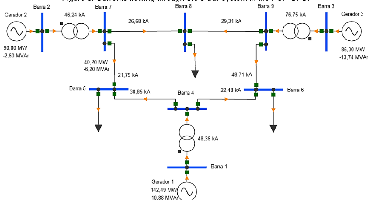
Figure 8: Currents flowing through the 9-bar system in the PSP-UFU.
