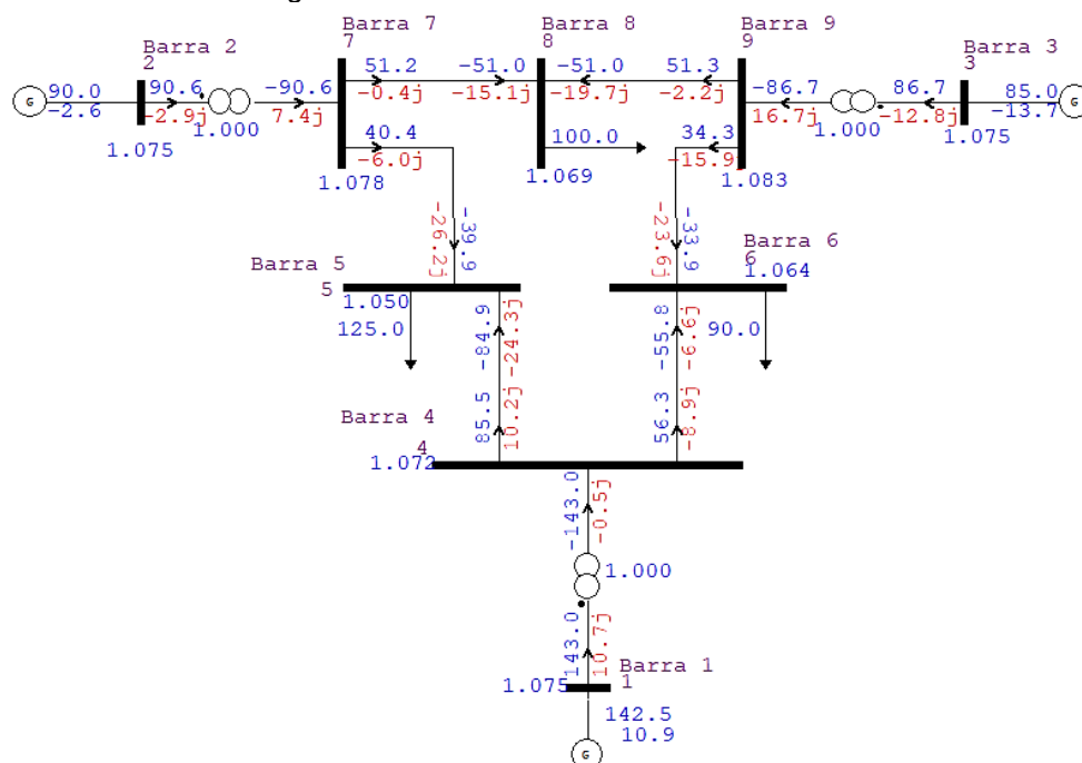
Figure 4: Circuit with load flow of ANAREDE.
