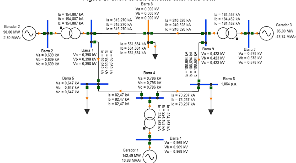
Figure 9: Short-circuit currents after load flow.
