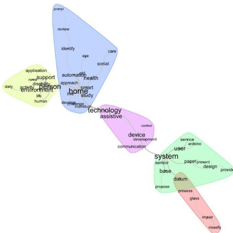
Figure 1. Similarity Analysis
