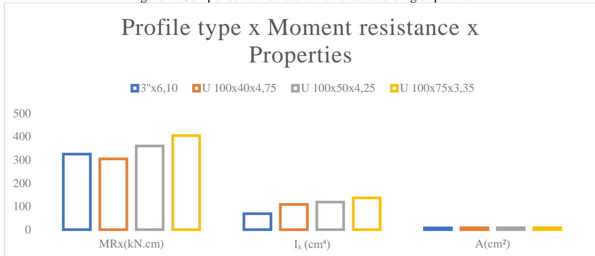
Figure 2: Comparison of resistant moments according to profile.
