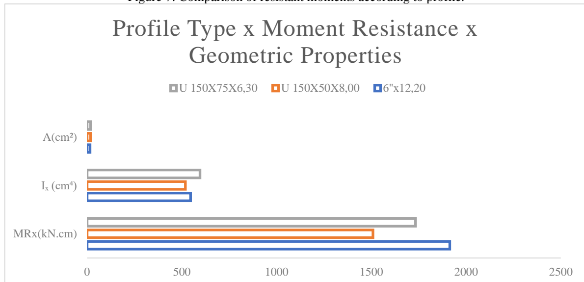
Figure 7: Comparison of resistant moments according to profile.
