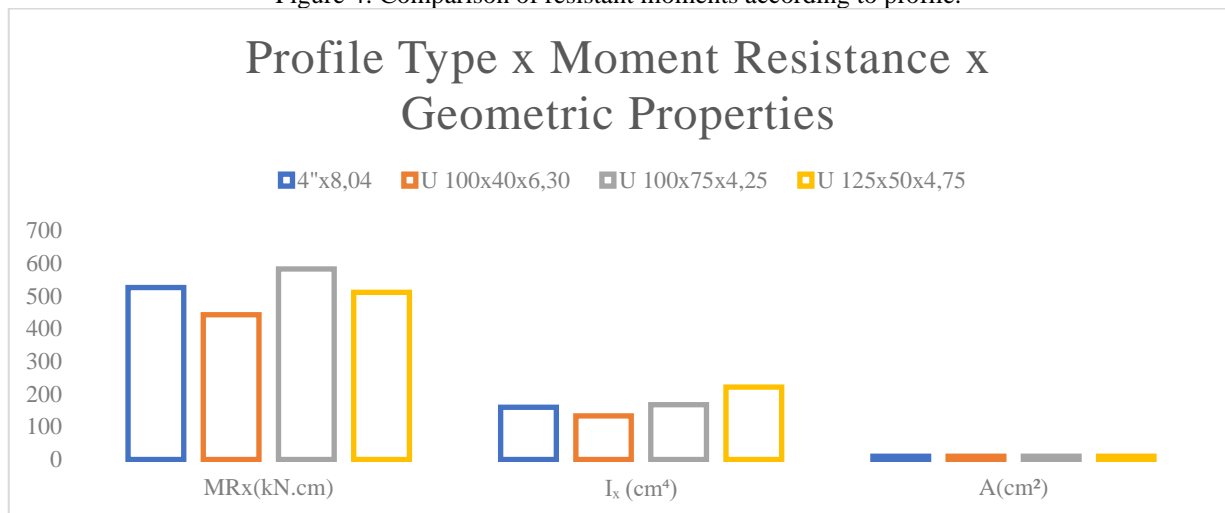
Figure 4: Comparison of resistant moments according to profile.
